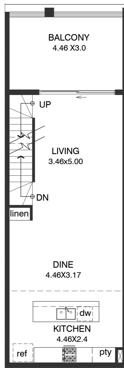
First Floor
