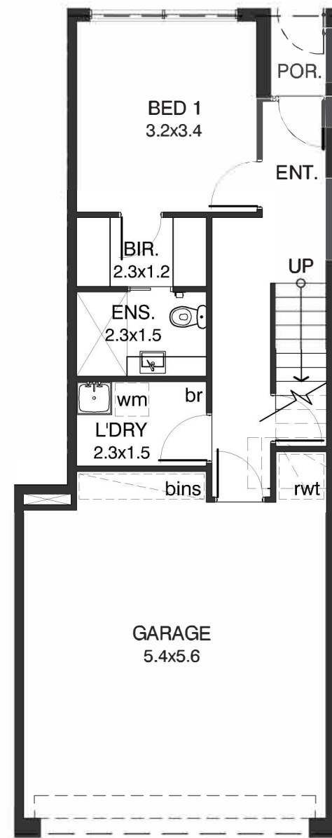
Ground Floor
