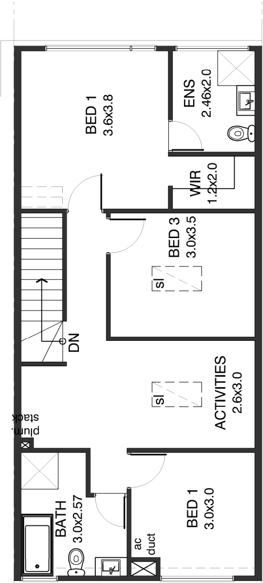
Second Floor
