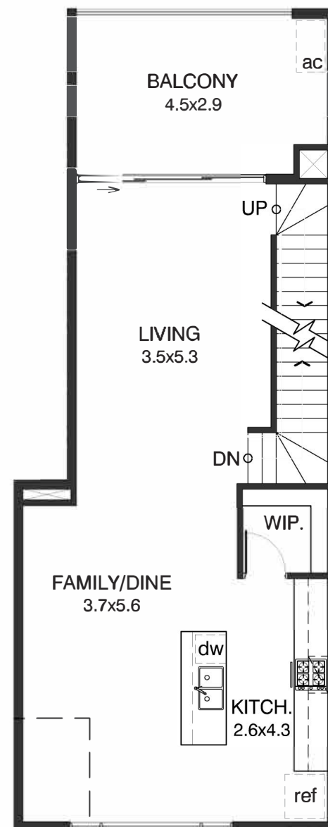
First Floor
